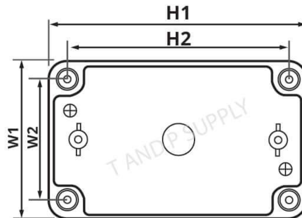
BASE
