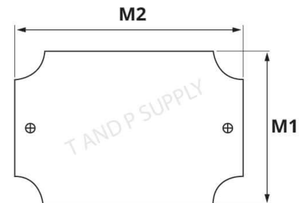
MOUNTING PLATE
